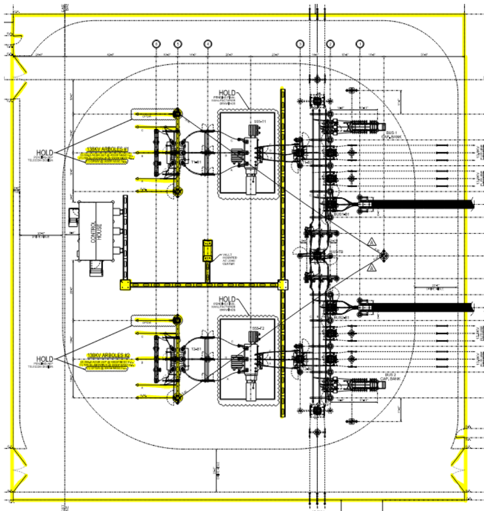
Figure 5: X-555 Above Grade Phase 1 install highlighted in yellow
