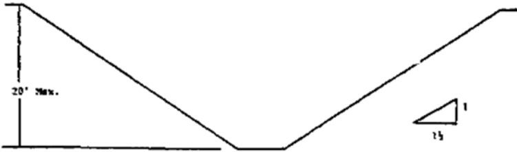
SIMPLE SLOPE – GENERAL FOR TYPE C SOIL
