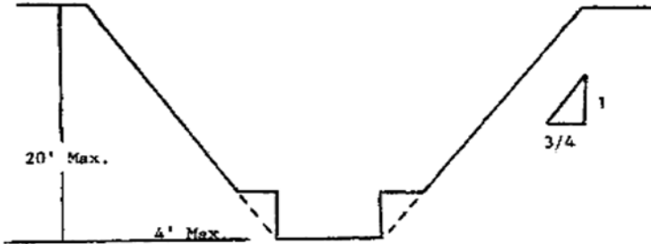
SIMPLE BENCH – GENERAL FOR TYPE A SOIL
