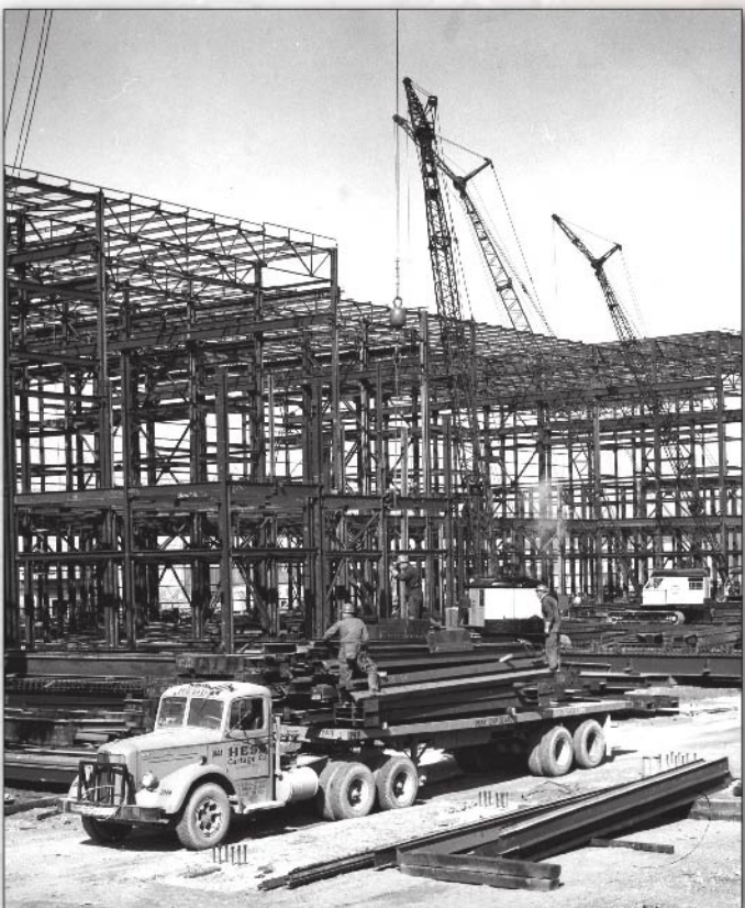
1954 Process building construction
